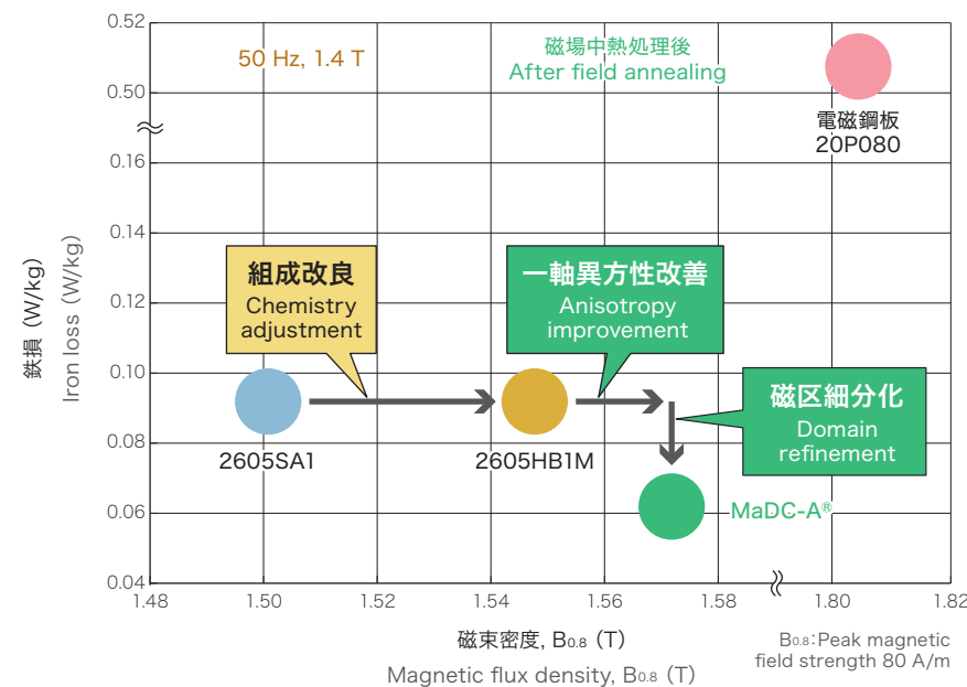
鉄損と磁束密度の関係(単板) Relationship between iron loss and magnetic flux density
